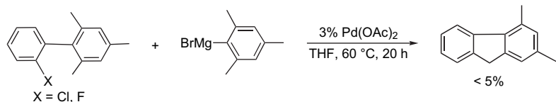
Scheme 5. Pd(OAc) 2 -catalyzed reactions of 2-halo-2',4',6'-trimethylbiphenyls with 2-mesitylmagnesium bromide.
