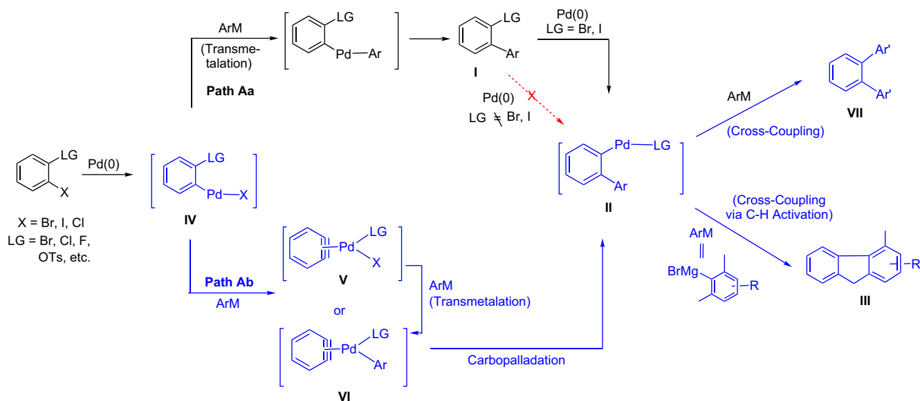
Scheme 4. Outline for 1-halo-2-(leaving group)benzenes for domino reactions via palladium(II)(LG)X associated aryne intermediates.
