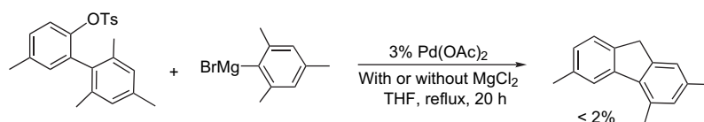
Scheme 10. Pd(OAc) 2 -catalyzed reaction of 2-(2',4',6'-trimethyl)-4-methylphenyl tosylate with 2-mesitylmagnesium bromide.
