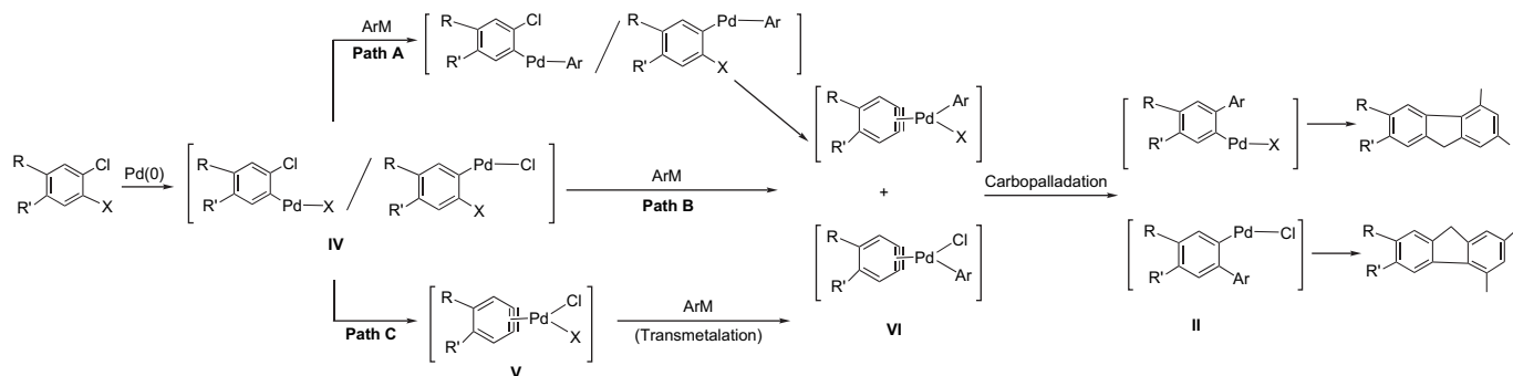
Scheme 7. Possible pathways for the formation of palladium(II)ClX associated aryne intermediates.
