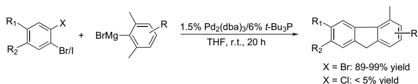
Scheme 2. Pd(0)/ t\text{-Bu}_3\text{P} -catalyzed tandem reactions of 1,2-dihaloarenes with hindered Grignard reagents.
