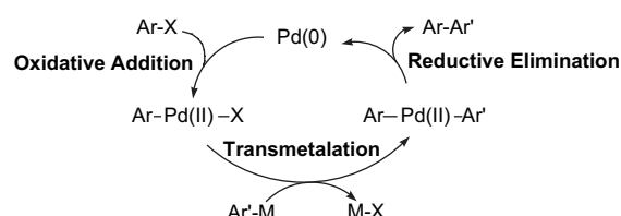
Figure 1. Generalized mechanism for Pd(0)-catalyzed cross-coupling reactions.
