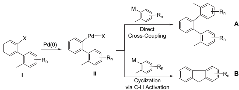
Scheme 1. Controlling competition between direct cross-coupling and cyclization via \text{sp}^3 C–H bond activation.
