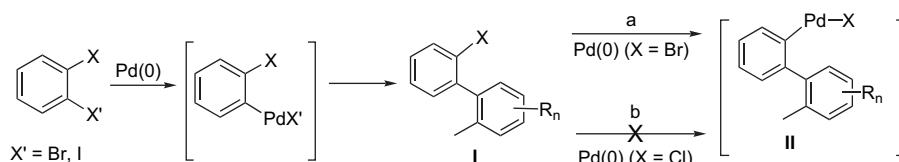
Scheme 3. Pd(0)/ t\text{-Bu}_3\text{P} -catalyzed tandem reactions of 1,2-dihaloarenes with bulky Grignard reagents.
