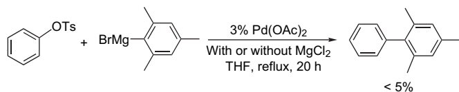
Scheme 9. Pd(OAc) 2 -catalyzed reaction of phenyl tosylate with 2-mesitylmagnesium bromide.
